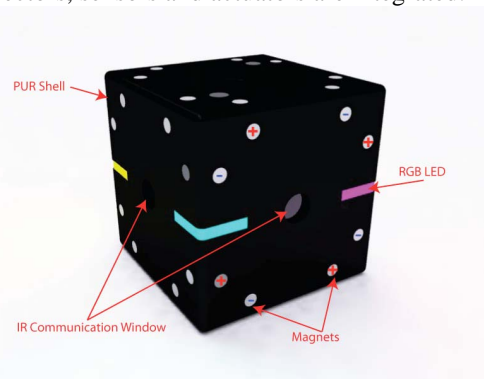
Figure 1. An explained visualization of the I-BLOCK.
